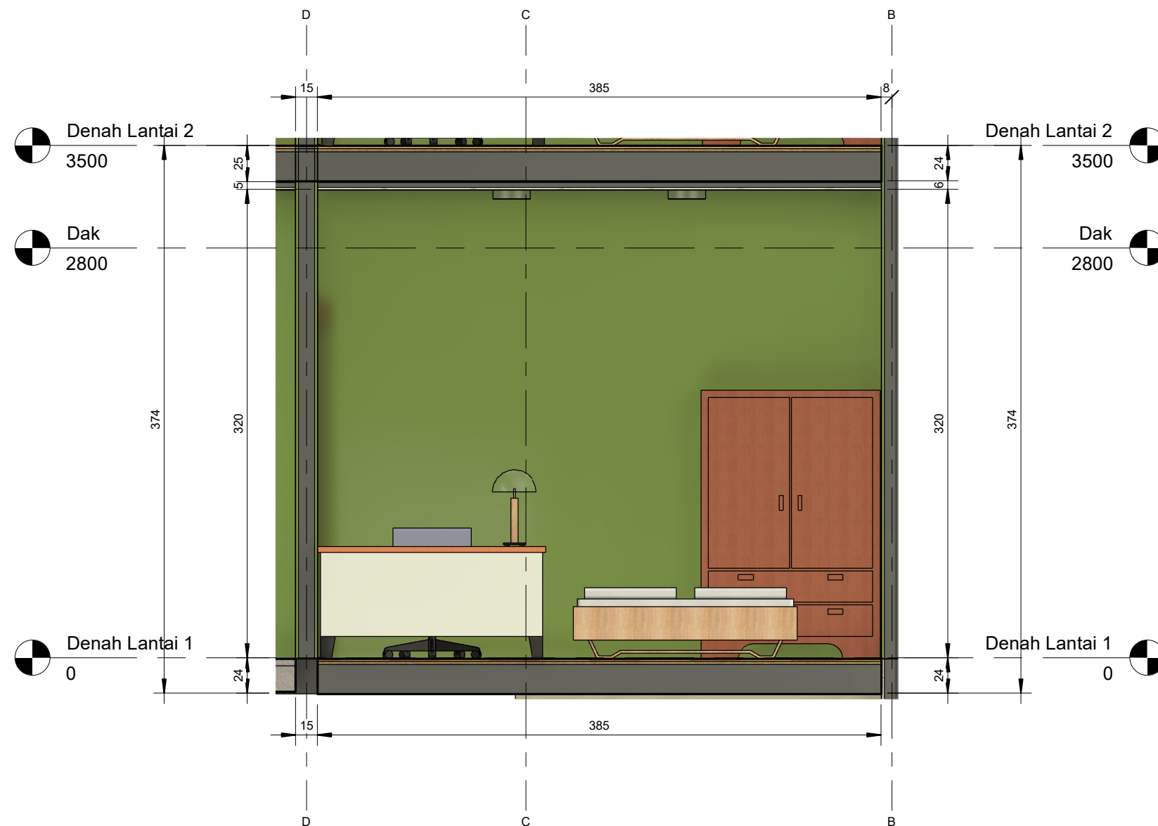
1 Kamar 1 - West 1 : 30
