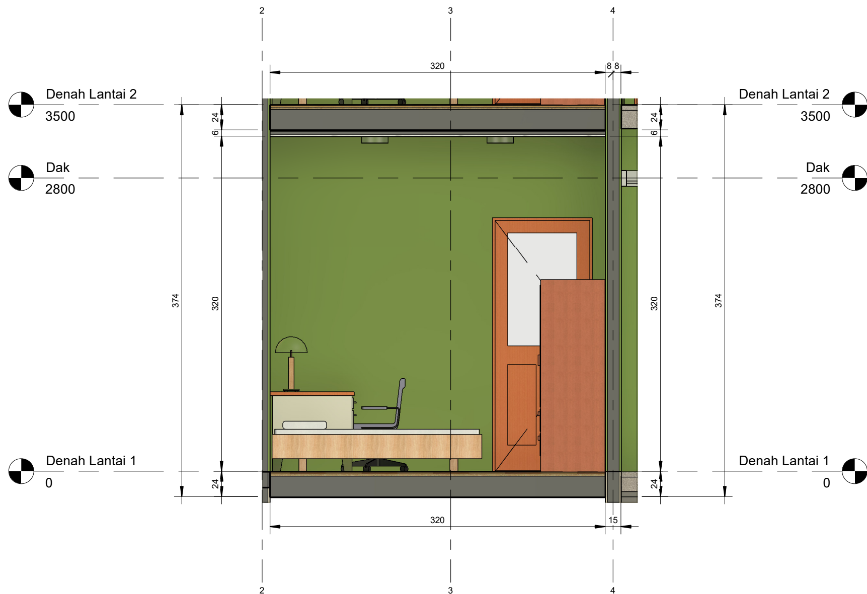
1 Kamar 1 - South 1 : 30
