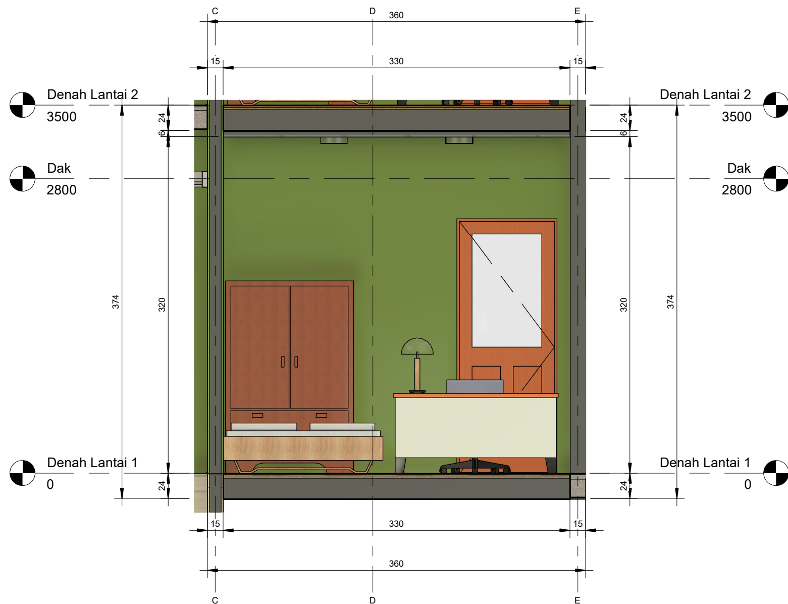
1 Kamar 2 - East 1 : 30
