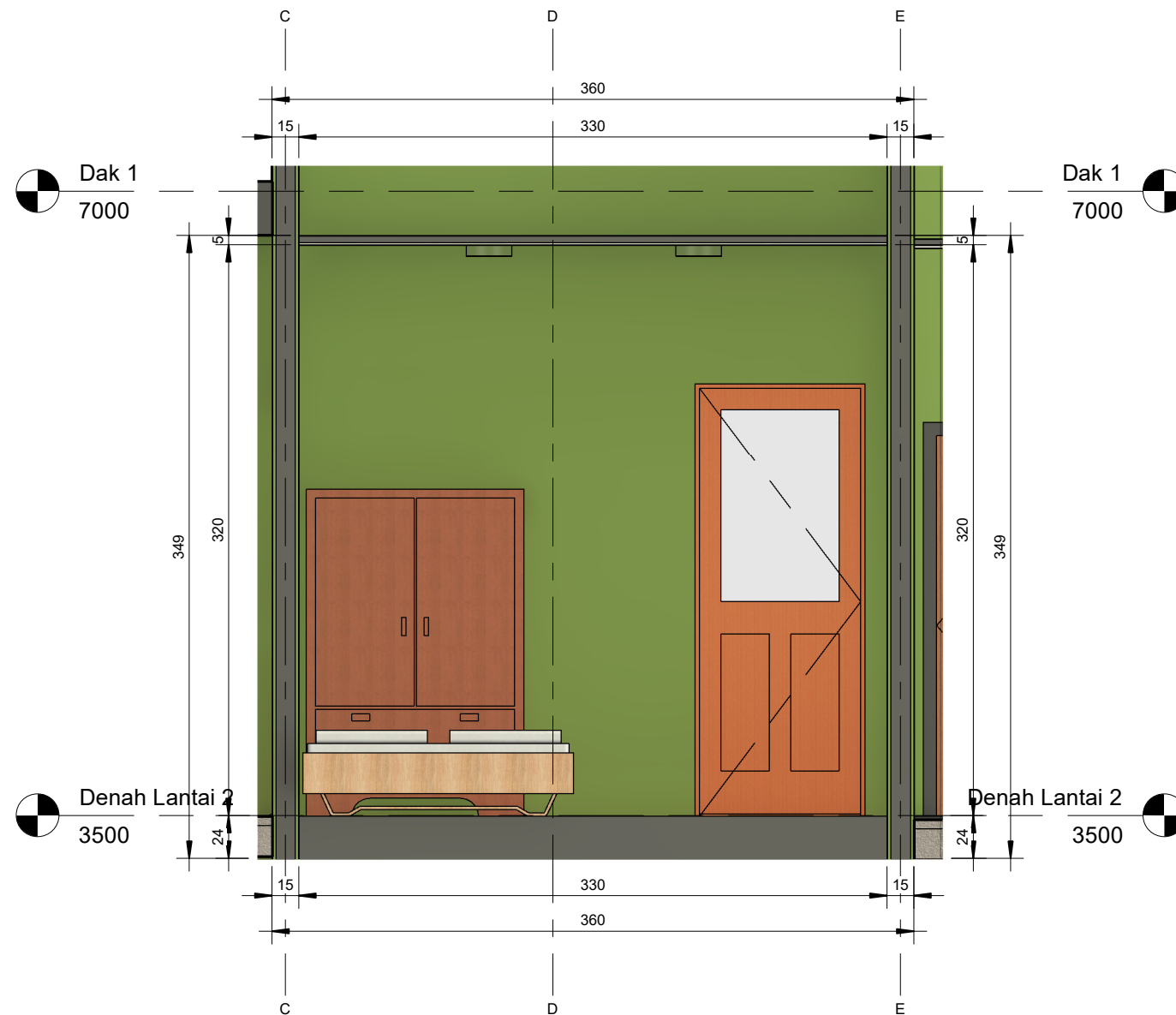
1 Kamar 4 - East 1 : 30
