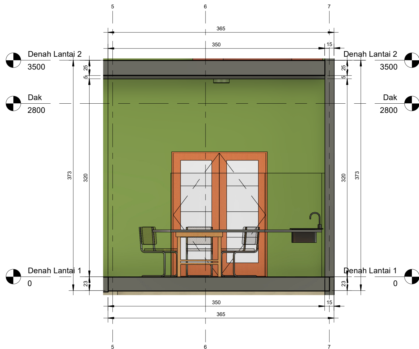
1 Dapur - South 1 : 30
