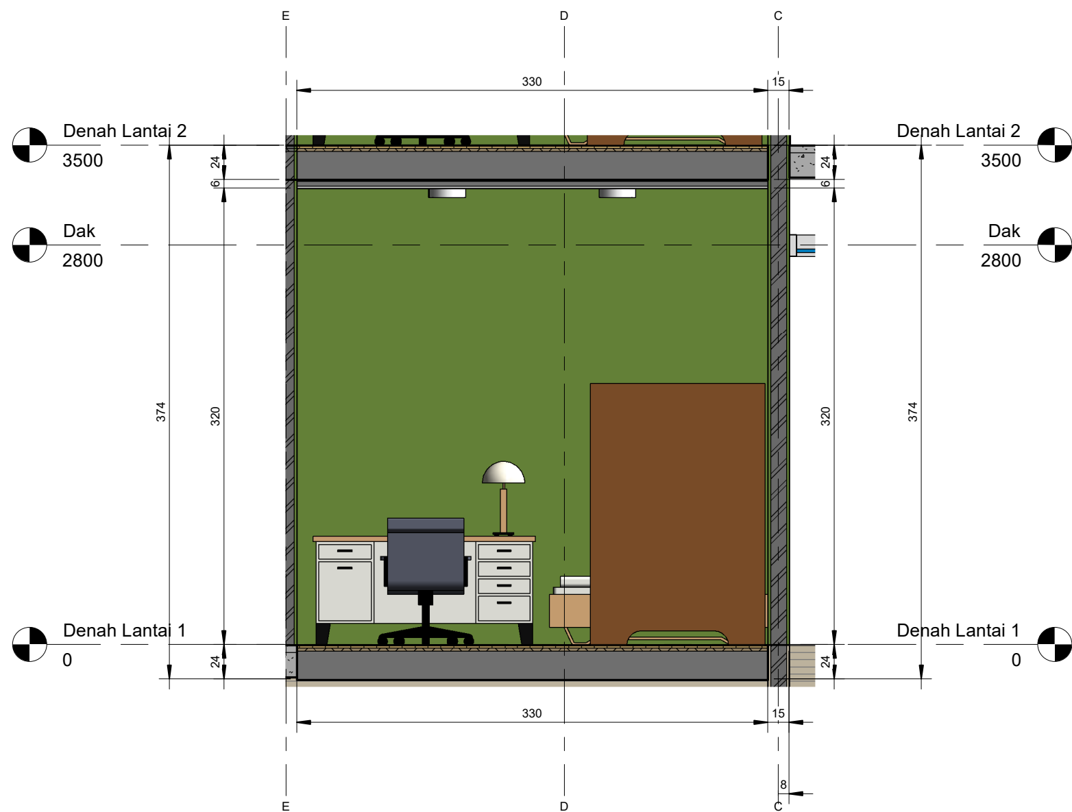
1 Kamar 2 - West 1 : 30
