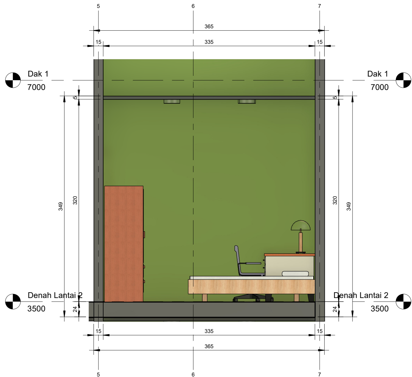
1 Kamar 4 - South 1 : 30
