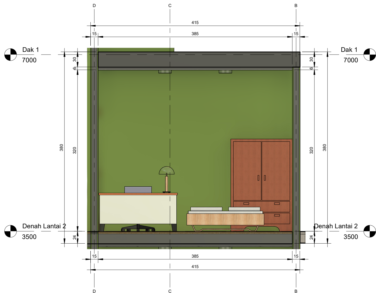
1 Kamar 3 - West 1 : 30
