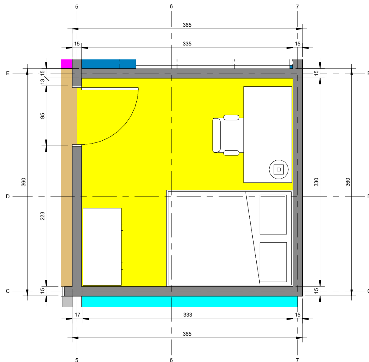
1 Denah Kamar 2 1 : 30
