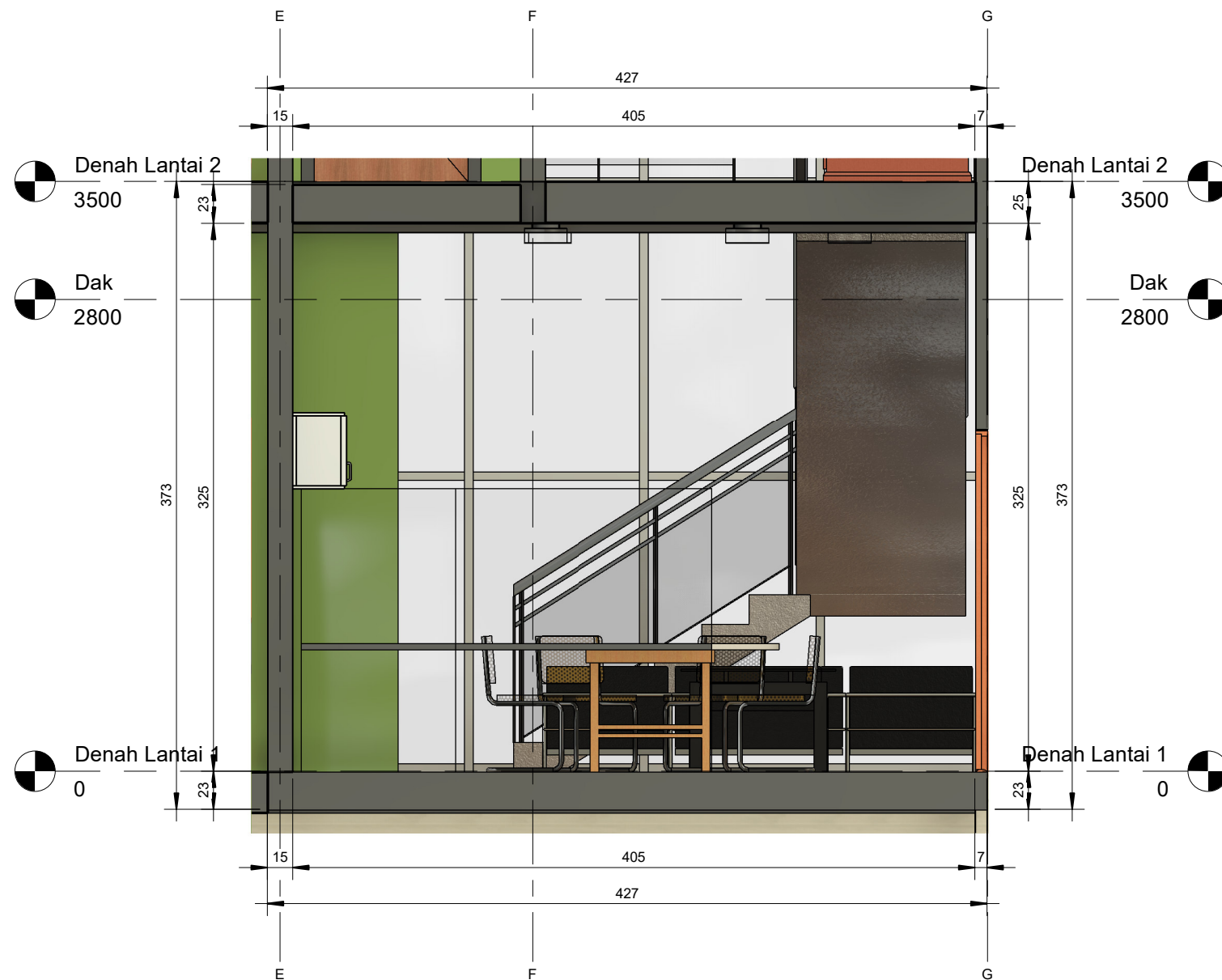
1 Dapur - East 1 : 30
