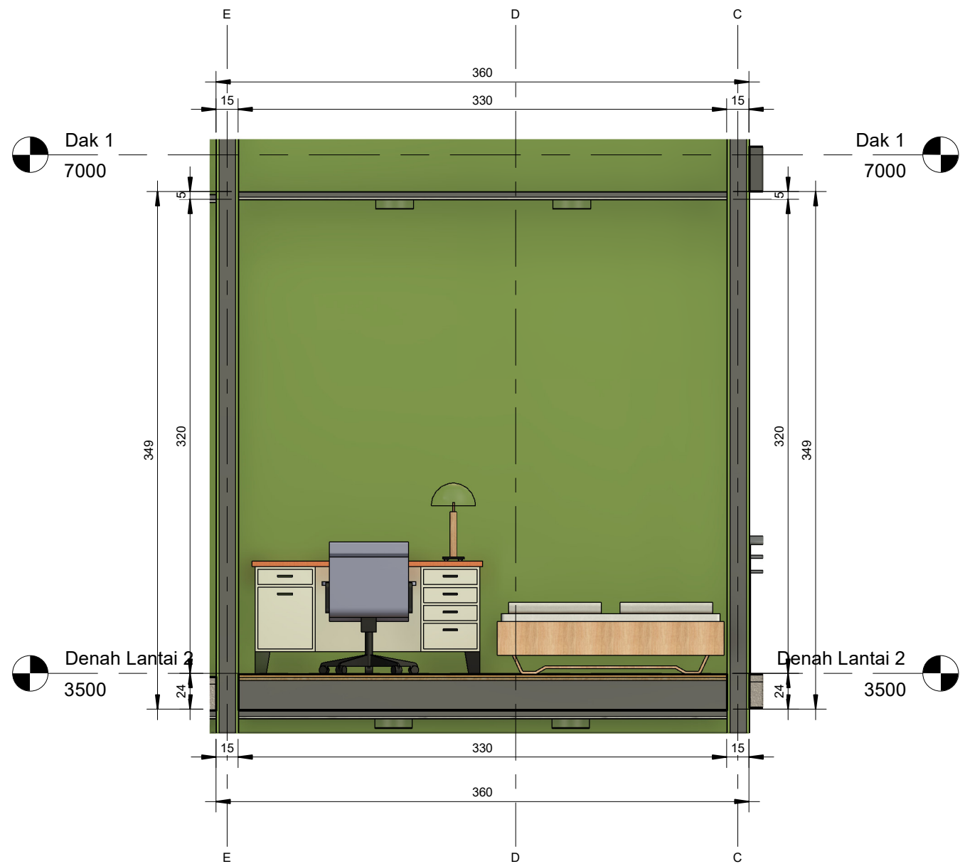
1 Kamar 4 - West 1 : 30
