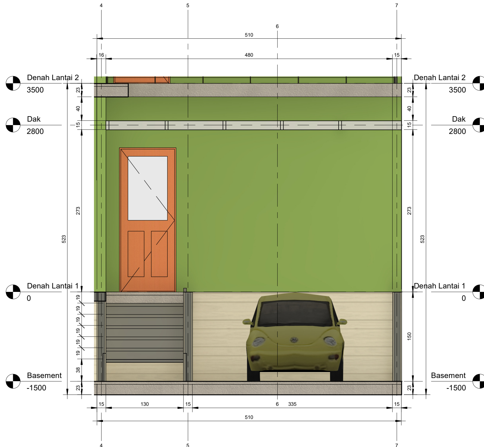
1 Carport - South 1 : 30
