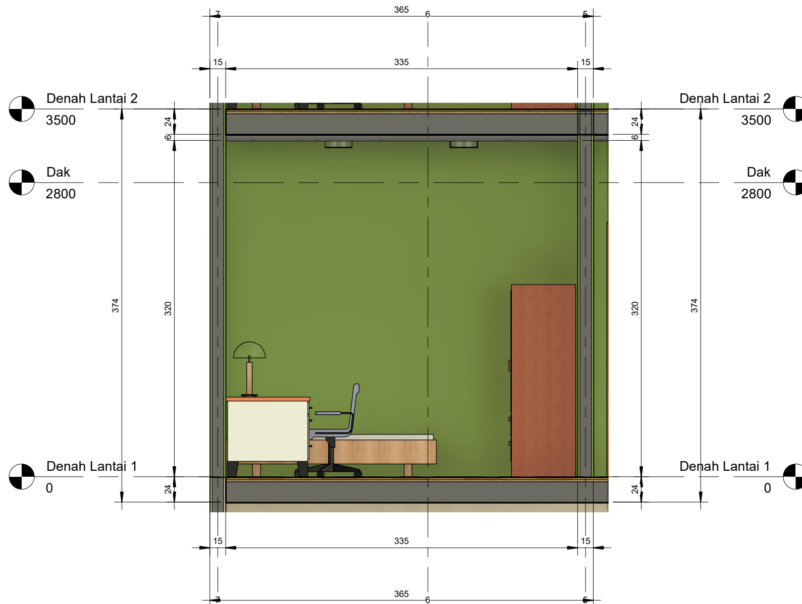
1 Kamar 2 - North 1 : 30
