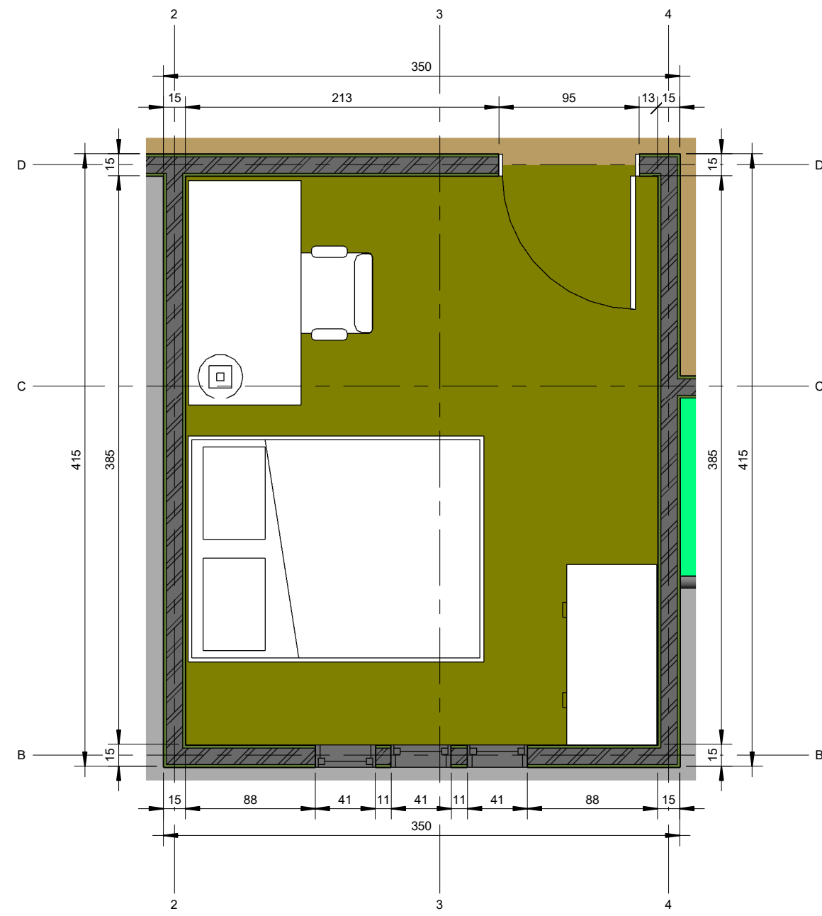
1 Denah Kamar 3 1 : 30
