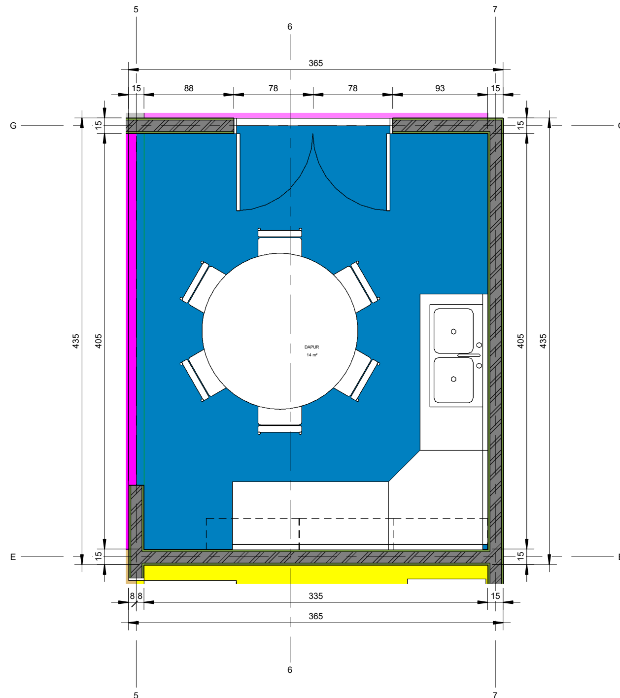
1 Denah Dapur 1 : 30
