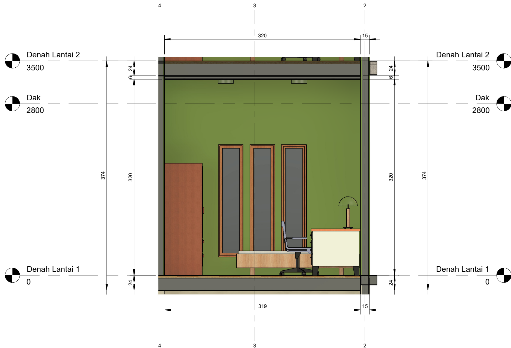
1 Kamar 1 - North 1 : 30
