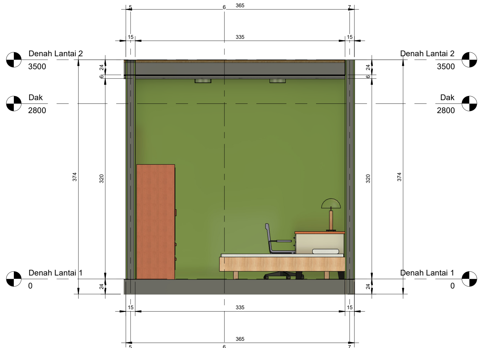
1 Kamar 2 - South 1 : 30
