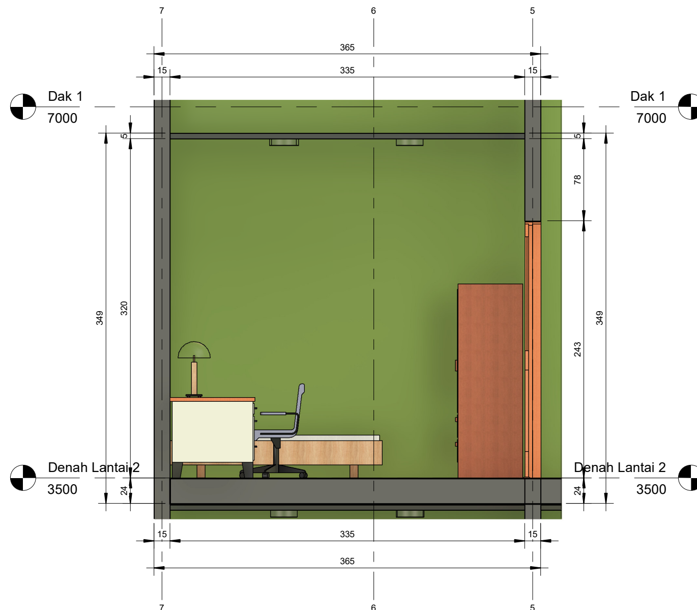
1 Kamar 4 - North 1 : 30
