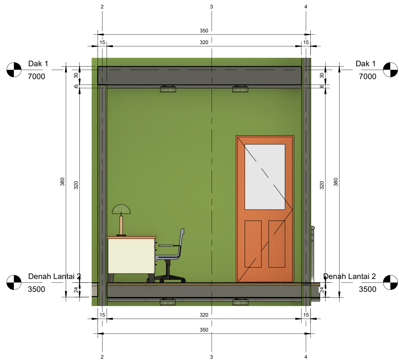
1 Kamar 3 - South 1 : 30
