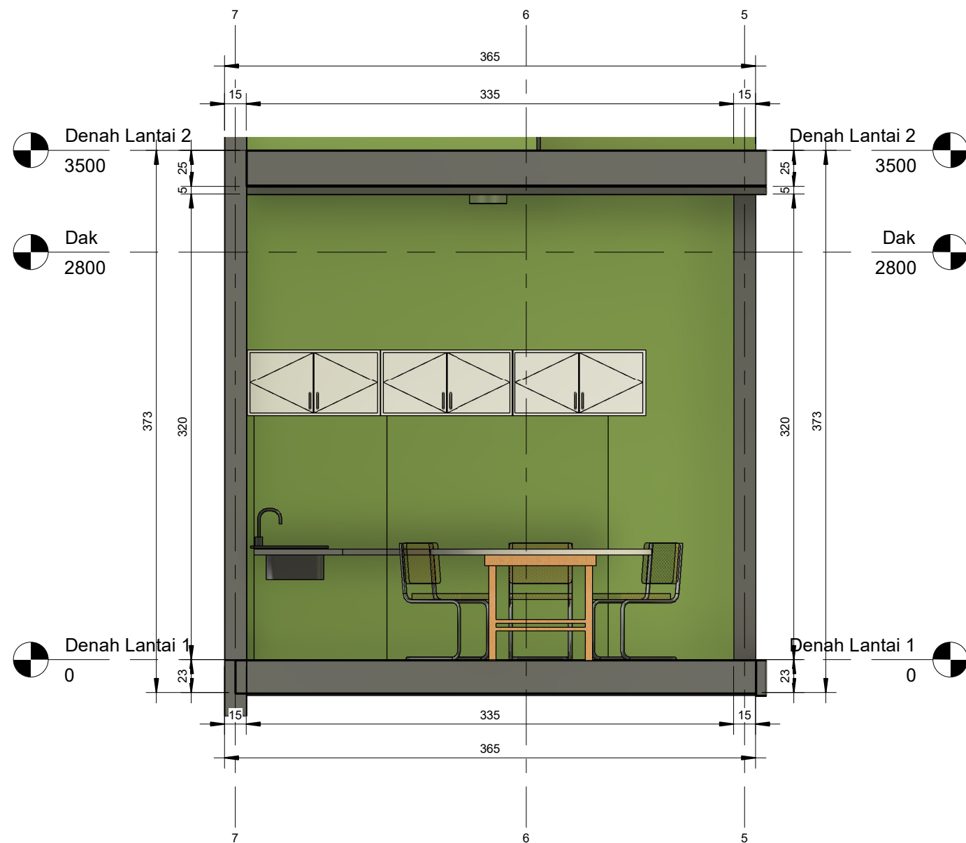
1 Dapur - North 1 : 30
