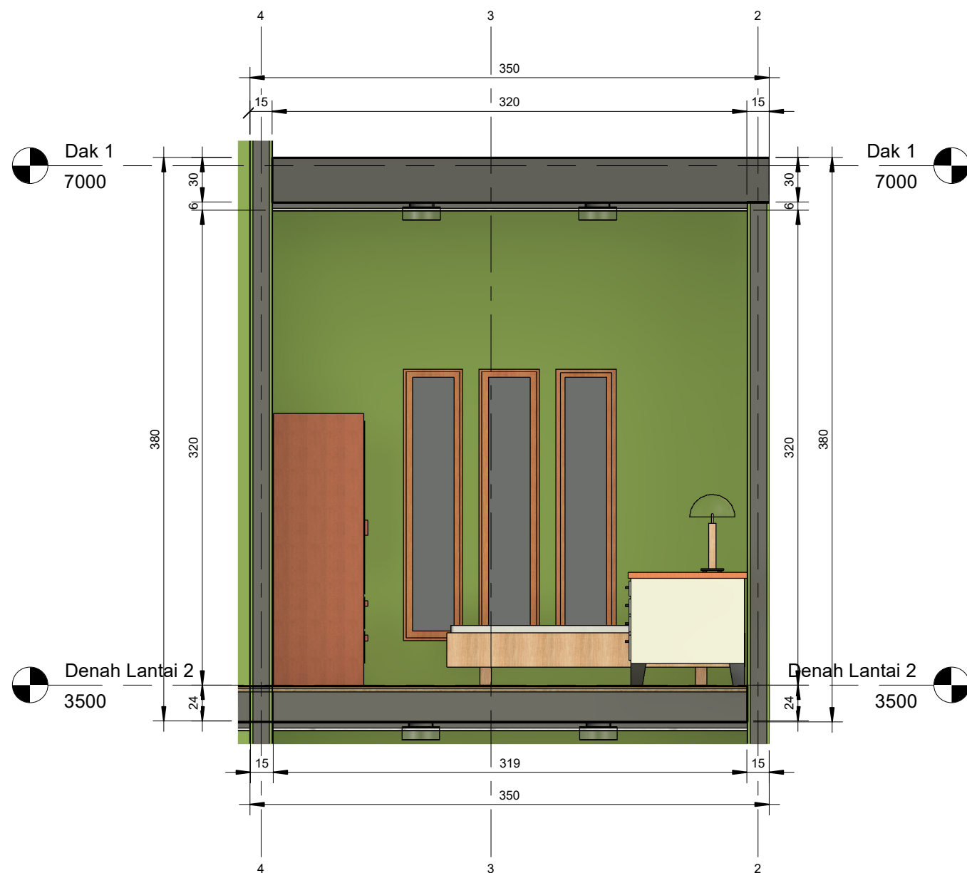
1 Kamar 3 - North 1 : 30
