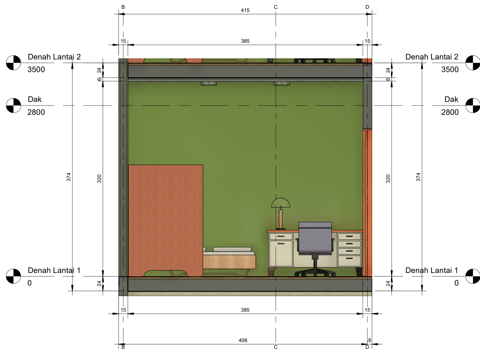
1 Kamar 1 - East 1 : 30
